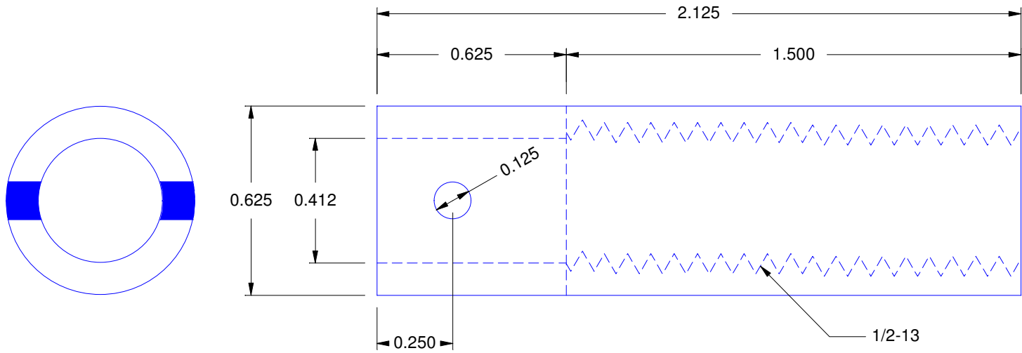
TRIM SCREW BARREL MATERIAL COLD ROLLED STEEL
