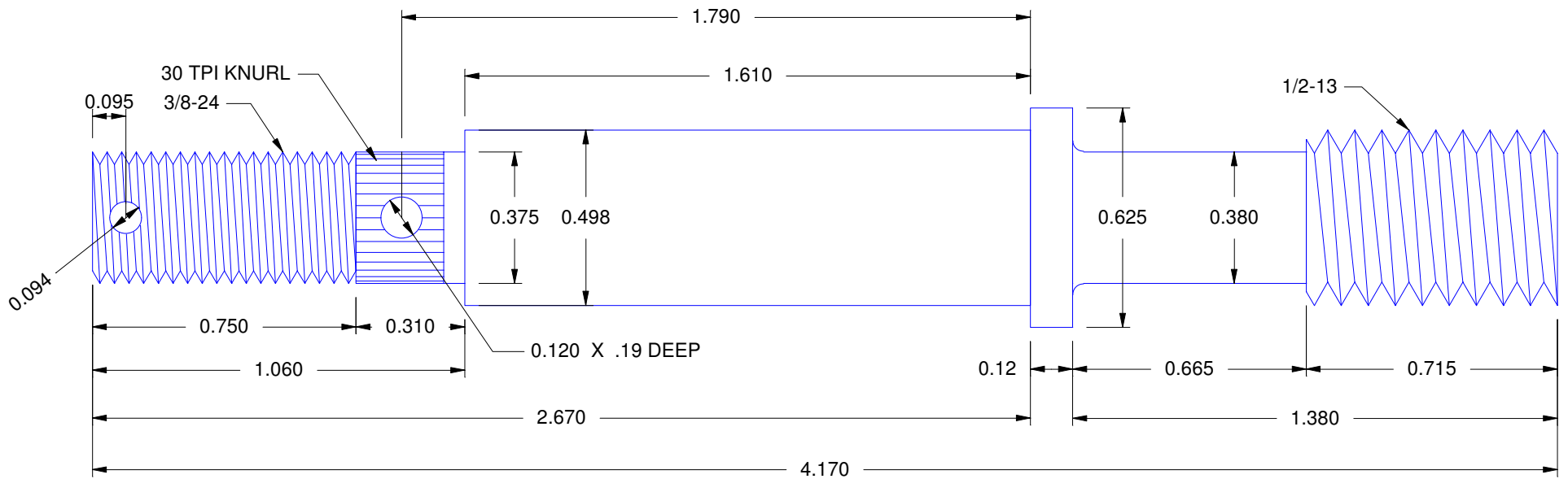
B12-406 TRIM SCREW MATERIAL 485 BRASS
