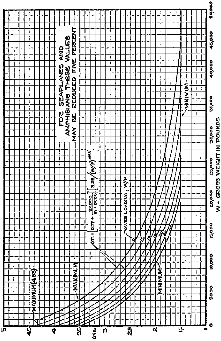
FIG. 04-3 MANEUVERING LOAD FACTOR INCREMENT, CONDITION I
