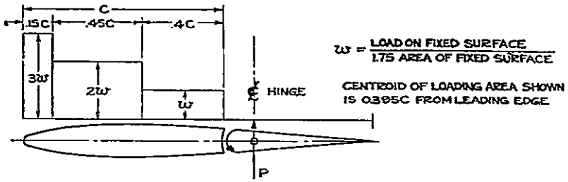
FIG. 04-4 "BALANCING" DISTRIBUTION - HORIZONTAL TAIL
