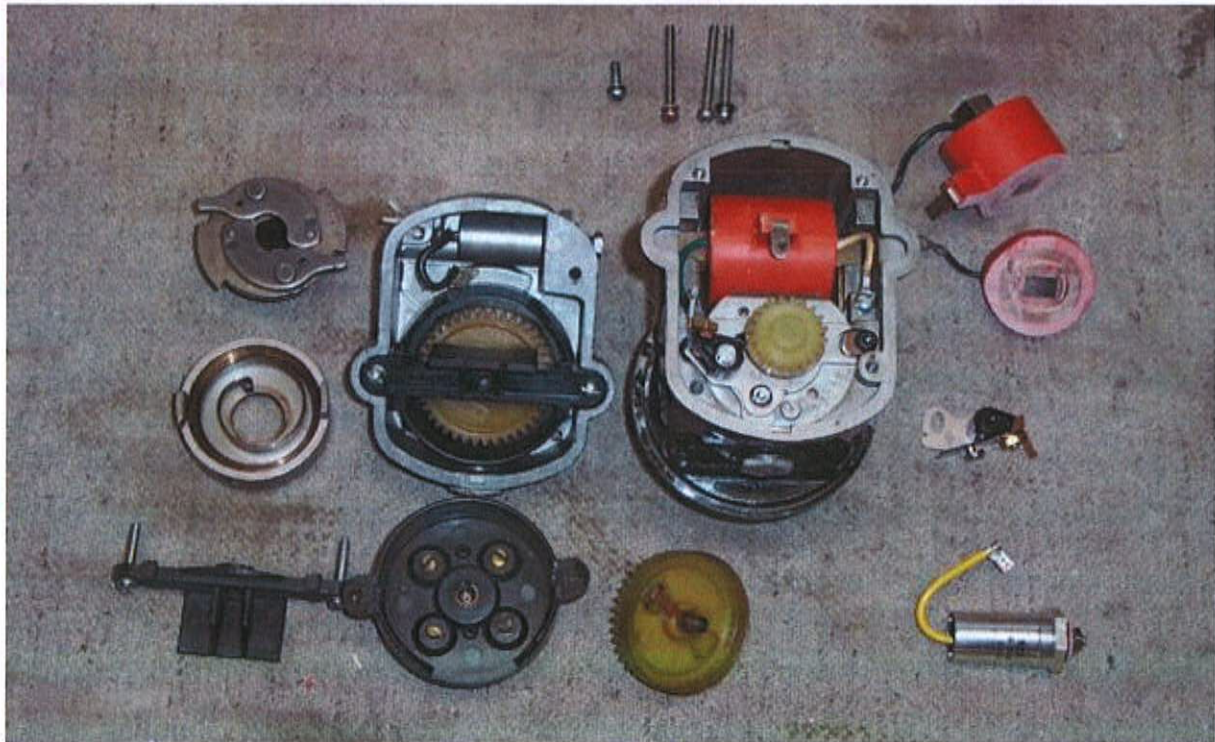
Photo 7: Here two ignition magnets have been disassembled completely.
